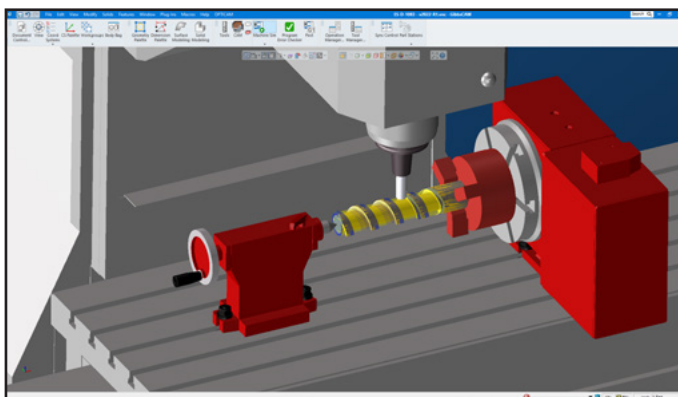
Radial milling
