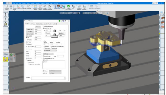
Directly machining 2.5D solids
