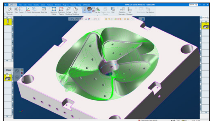
3D machining
